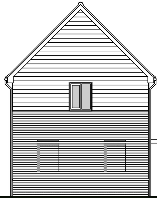
Side Elevation (Additional Side windows 10, 29, 57 )
