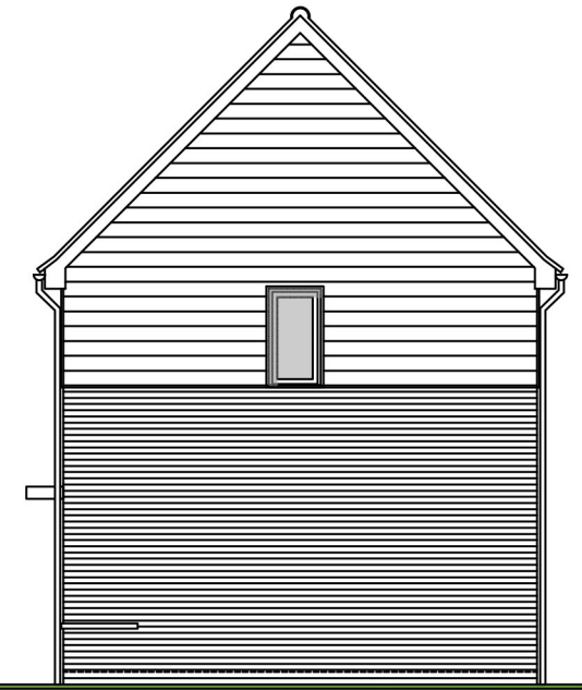
Side Elevation (Additional Side windows 20, 38, 119 )
